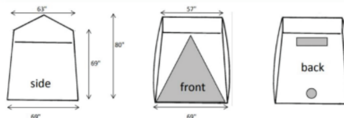
SPECIFICATIONS - 6' x 6' FOOTPRINT
